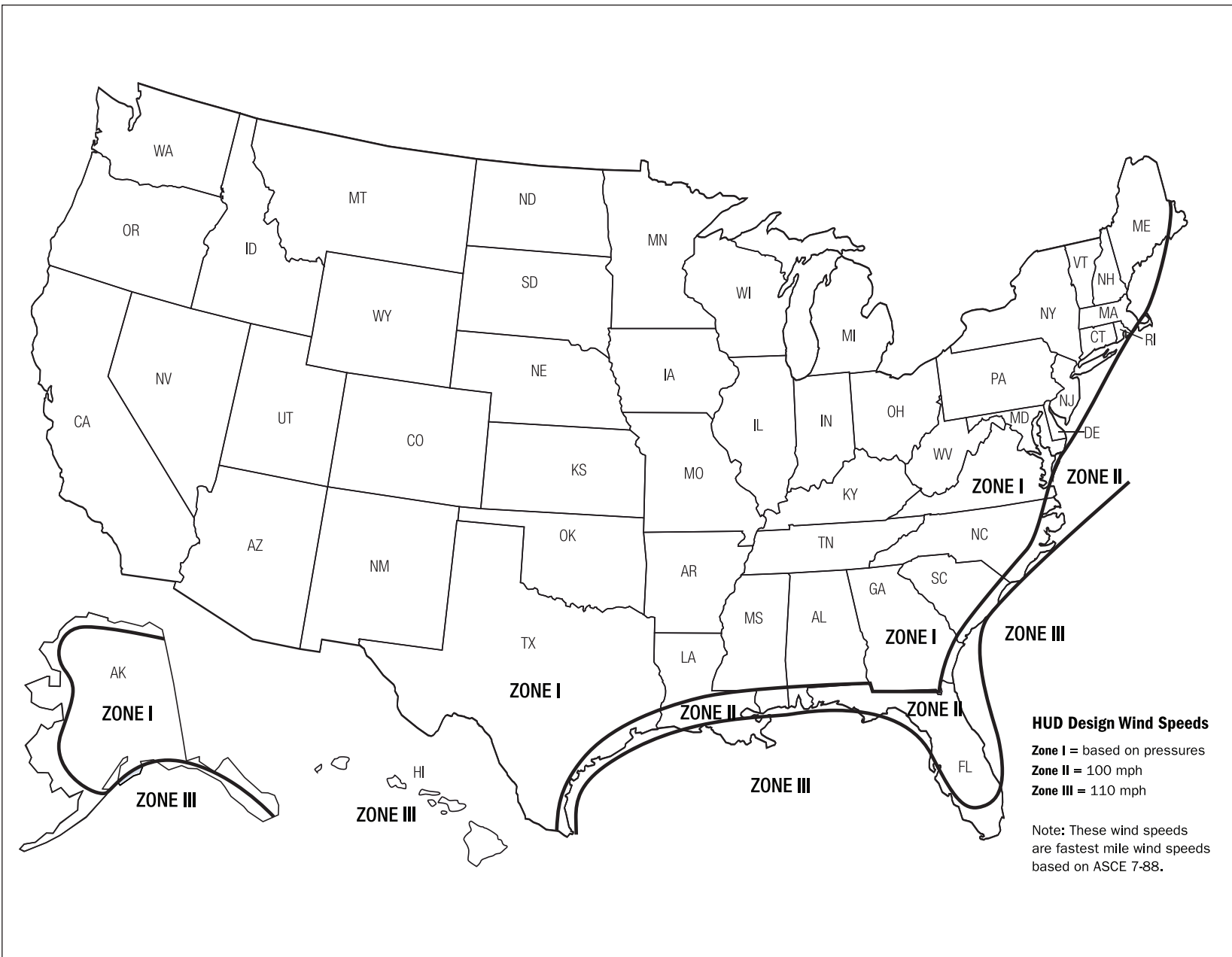
Figure 1-1. Basic wind zone map for manufactured housing.
