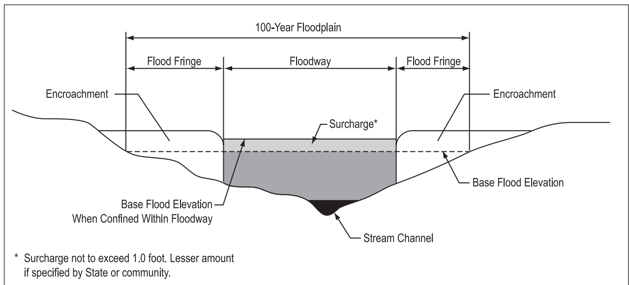
Figure 4-2. Floodplain/floodway schematic.
