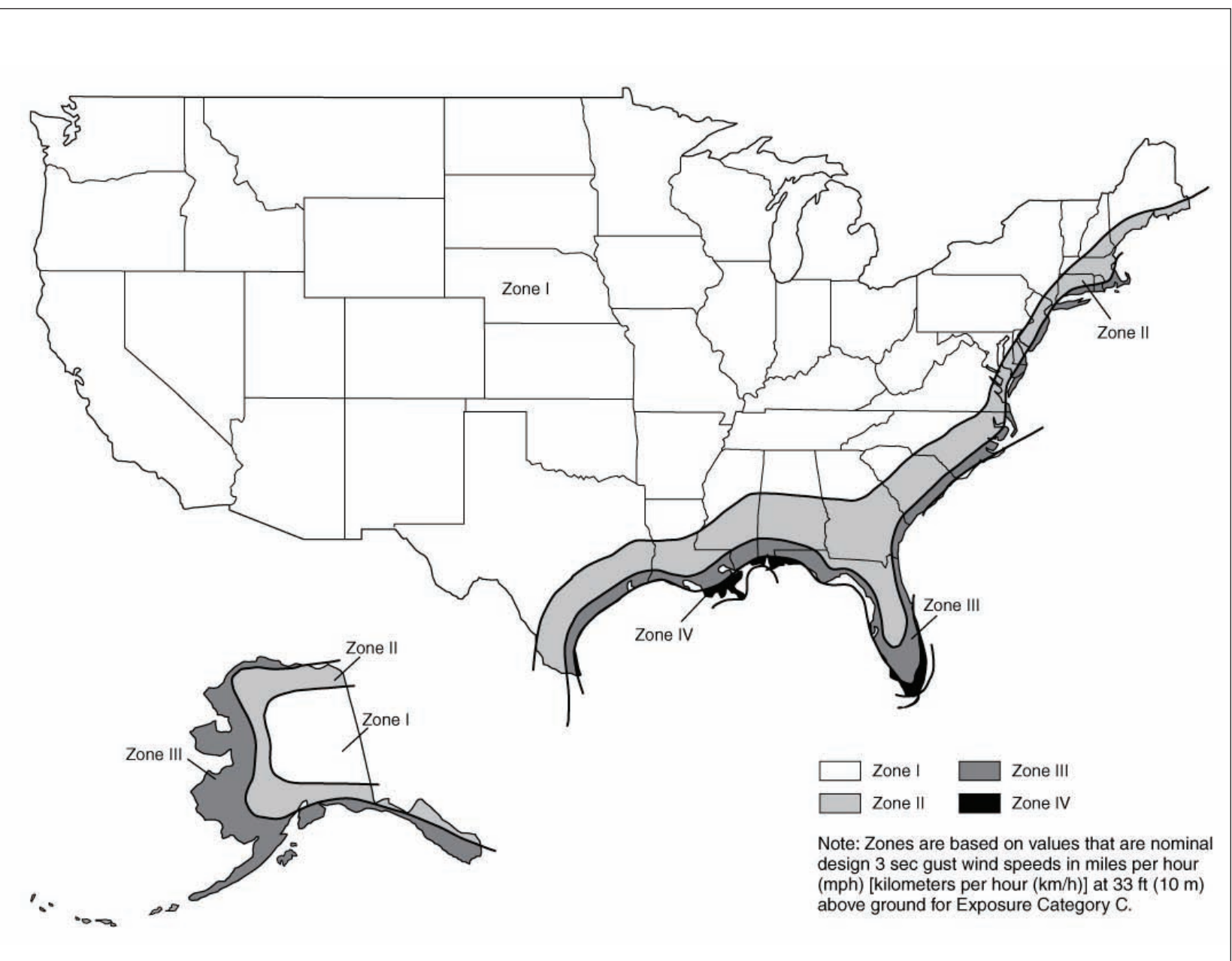
Figure G-2. NFPA 501 wind speed map.
