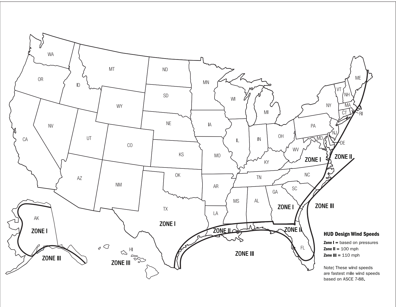
Figure G-1. Basic wind zone map for manufactured housing.
