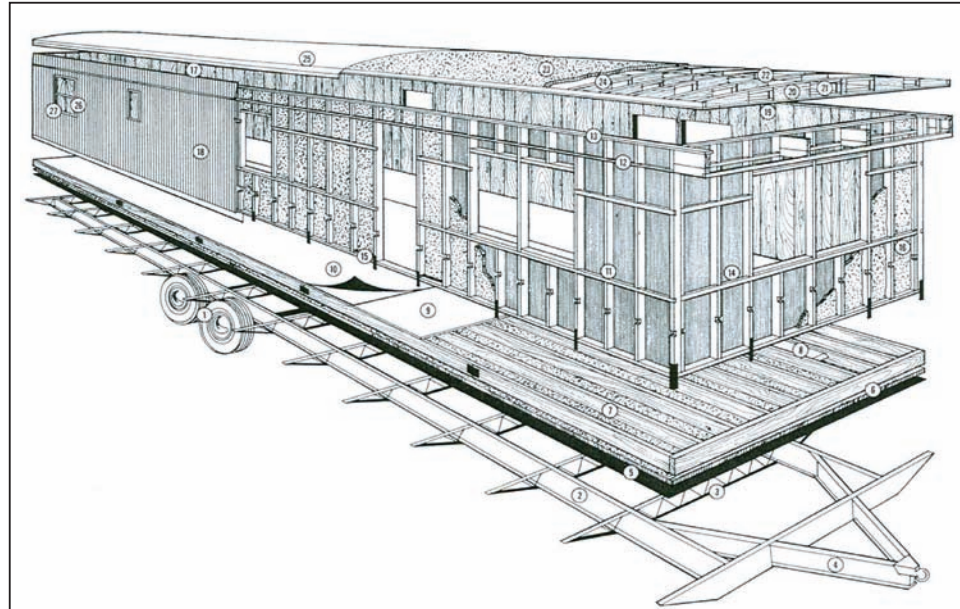
Figure 2-3. Main construction features of a typical manufactured home.
